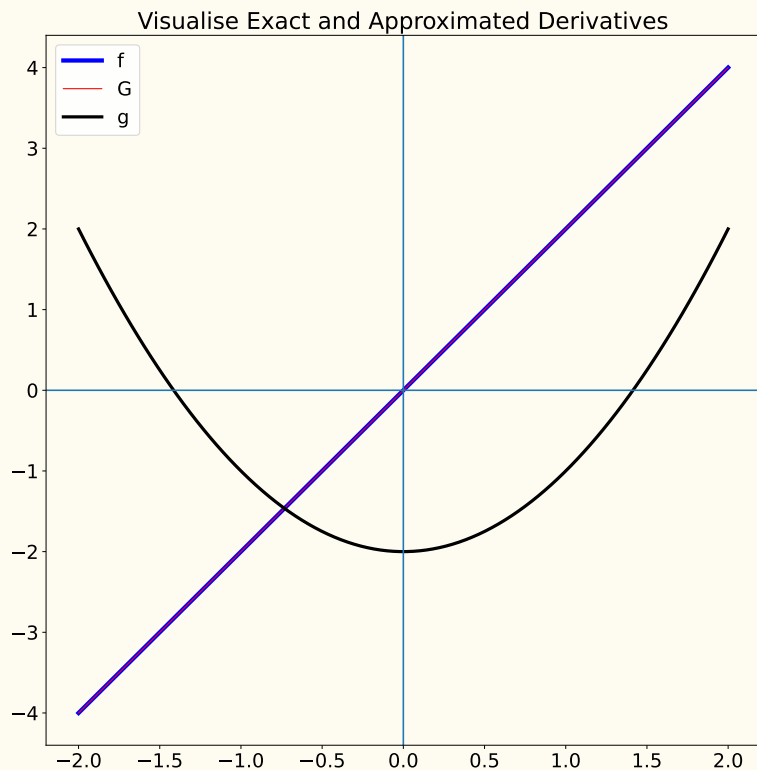
Figure 3: matplotlib visualisation
