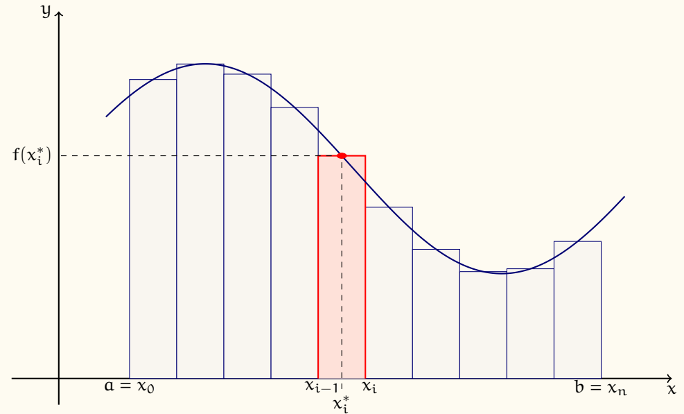
Figure 4: General idea of Riemann integration
